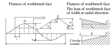
Figure 4 Flatness Requirement
